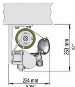
Soffit Mount
