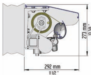
Wall Mount
