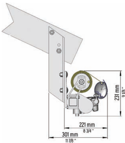
Joist Mount
