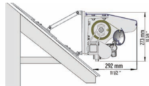
Roof Mount
