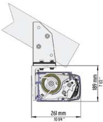
Joist Mount
