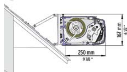
Roof Mount
