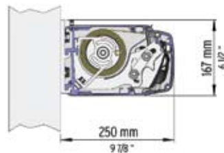
Wall Mount
