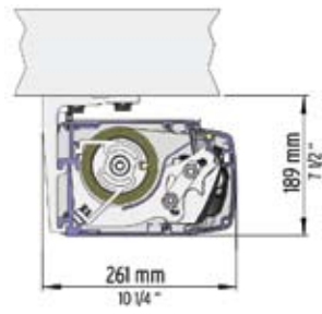
Soffit Mount
